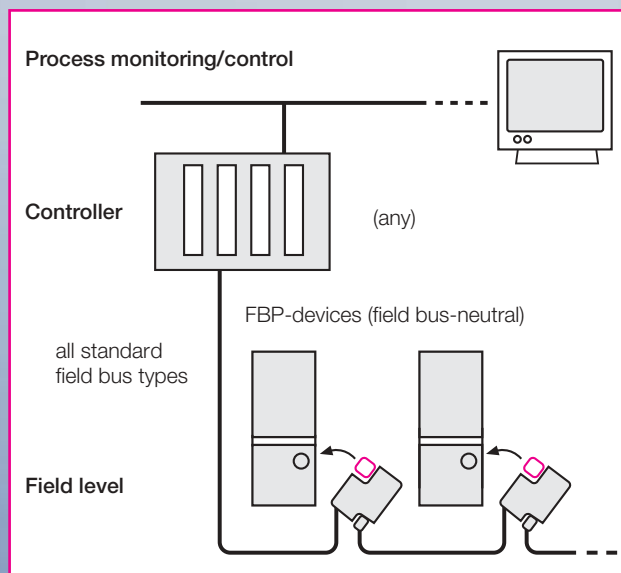
Installation principle
